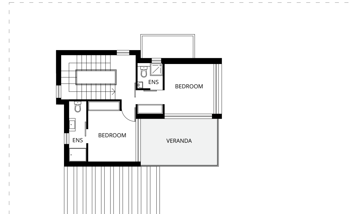
FIRST FLOOR
